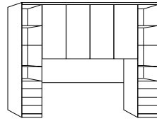
Overbed unit in carcass colour, with towers 40 cm in carcass colour, 4 drawers underneath, above open compartment and 2 wooden shelves, W 230 cm for bed width 140 cm W 250 cm for bed width 150/160 cm W 270 cm for bed width 180 cm
