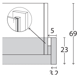
Top view wardrobe incl. PPT-Frame
