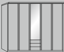
Combi wardrobes* with wooden or mirrored doors and 3 drawers, incl. cornice, W 33-400 cm, H 220/240 cm, D 58 cm
