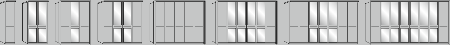
Hinged-door wardrobes doors in carcass colour, with or without centre doors in mirrored glass, W 50 – 400 cm, H 220 cm, D 58 cm
