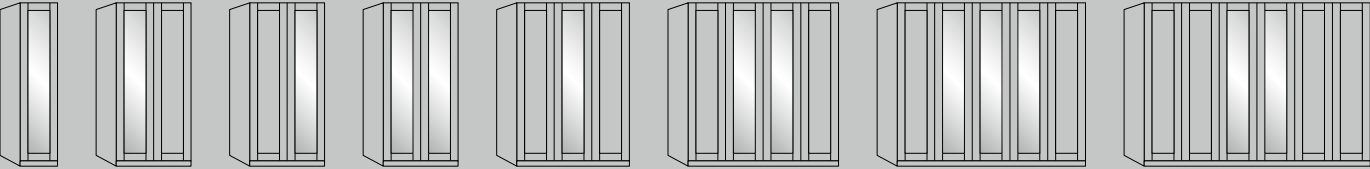
Hinged-door wardrobes doors in carcase colour with or without mirrored glass, W 50 – 300 cm, H 216 cm, D 58 cm
