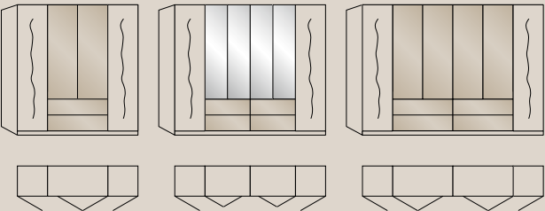
Combi wardrobes with bi-fold-panorama doors with 2 or 4 drawers outer doors in heartwood veneer, centre door/s and drawers in glass or centre door/s in mirror and drawers in glass, W 200 – 300 cm, H 216/236 cm, D 58 cm
